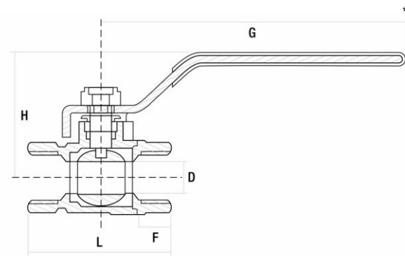
HEAVY BRASS BALL VALVE WITH SS HANDLE, NY LOCK NUT (SS)
