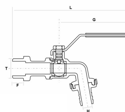
NOZZLE BRASS BIB COCK WITH STAINLESS STEEL HANDLE
